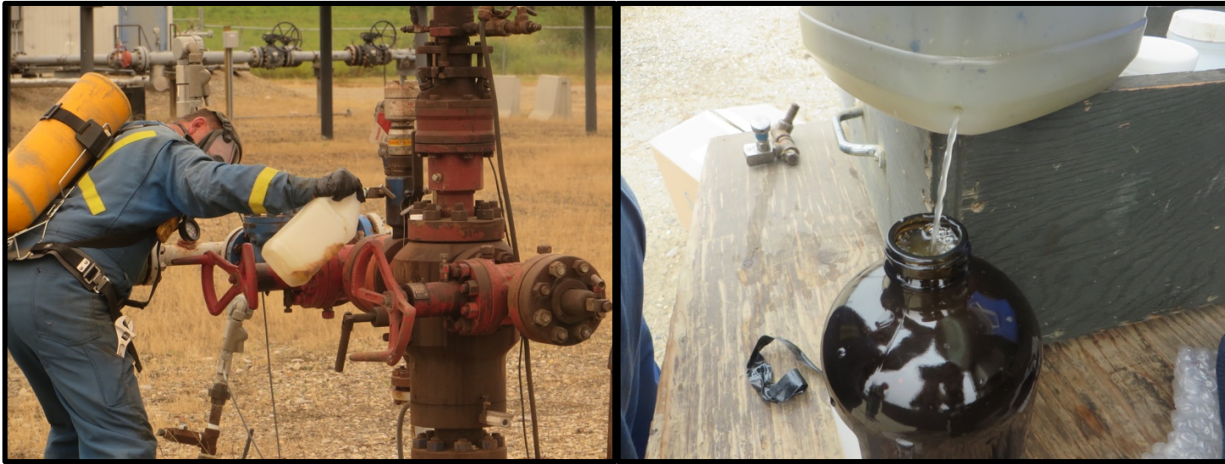
Figure 11: Sample collection at wellhead. Left: Maxxam employee sampling from access port into 4 L plastic container. Right: Decanting brine sample from bottom of 4 L container.
