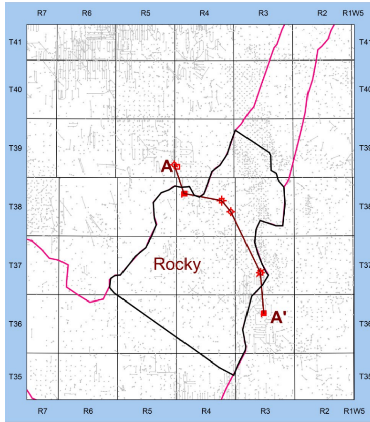
Figure 8: Area map (GeOLOGIC Systems) of the NRRA (black), the regional Leduc edge (Pink) and cross section reference lines (burgundy) for Figures 9 and 10 (E3 Metals Corp, 2017).
