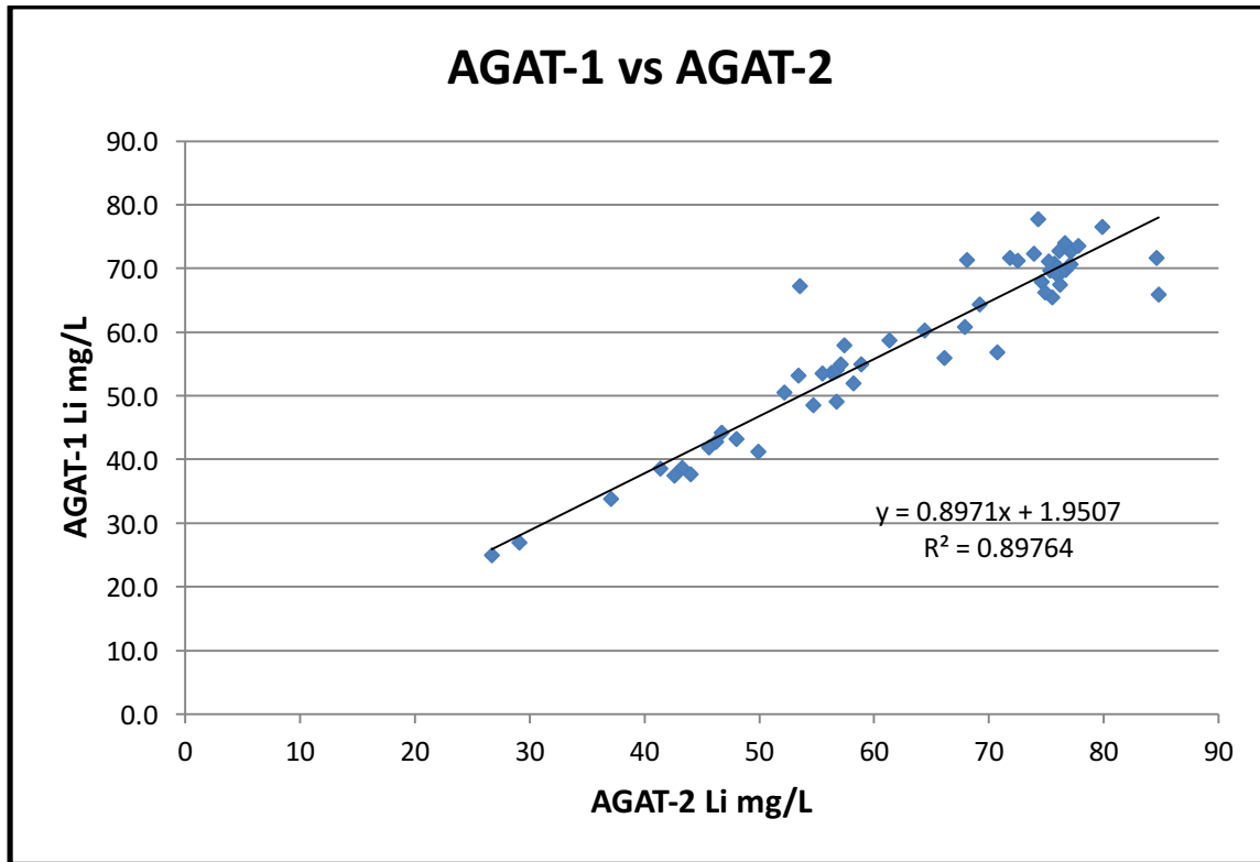
Figure 15. Scatter plot of duplicate Li-brine well sample analyses from AGAT laboratory.
