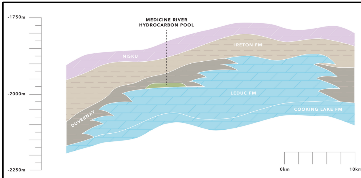
Figure 10: Schematic representation of the NRRRA (to scale with vertical exaggeration) highlighting the relationships of the geology, structure, and hydrocarbon pools (E3 Metals, 2017)
