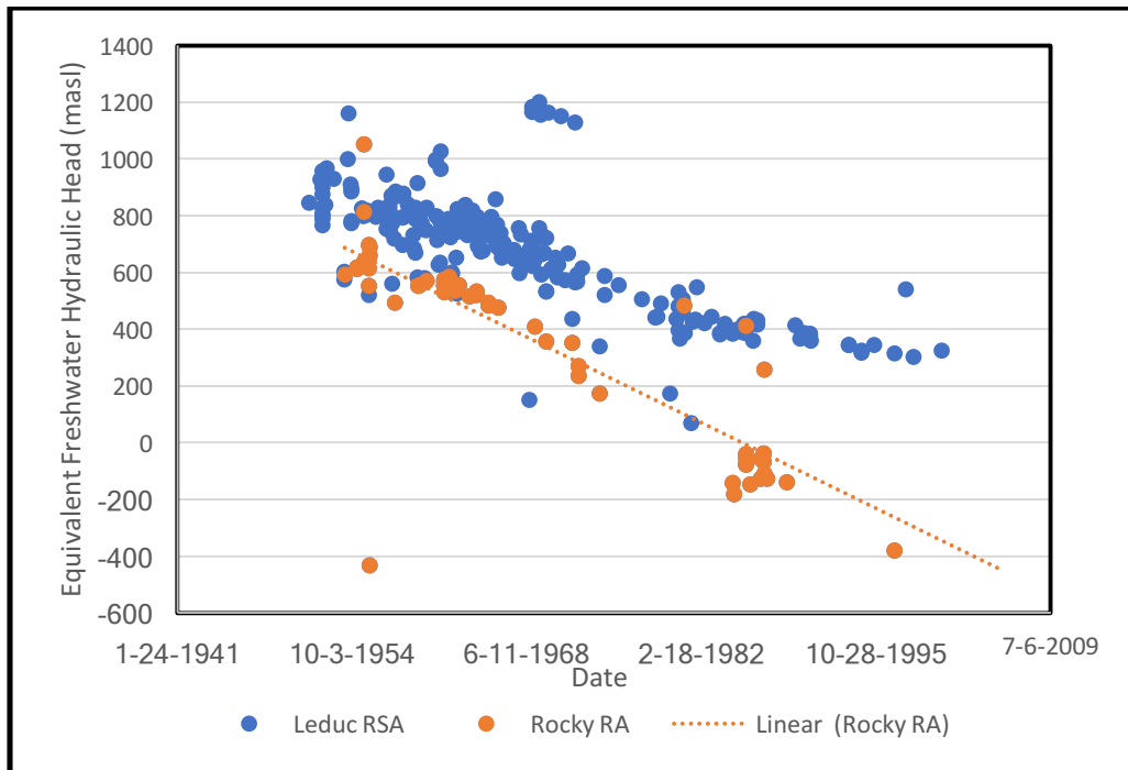
Figure 25. NRRRA DST derived hydraulic heads over time as compared to regional data.
