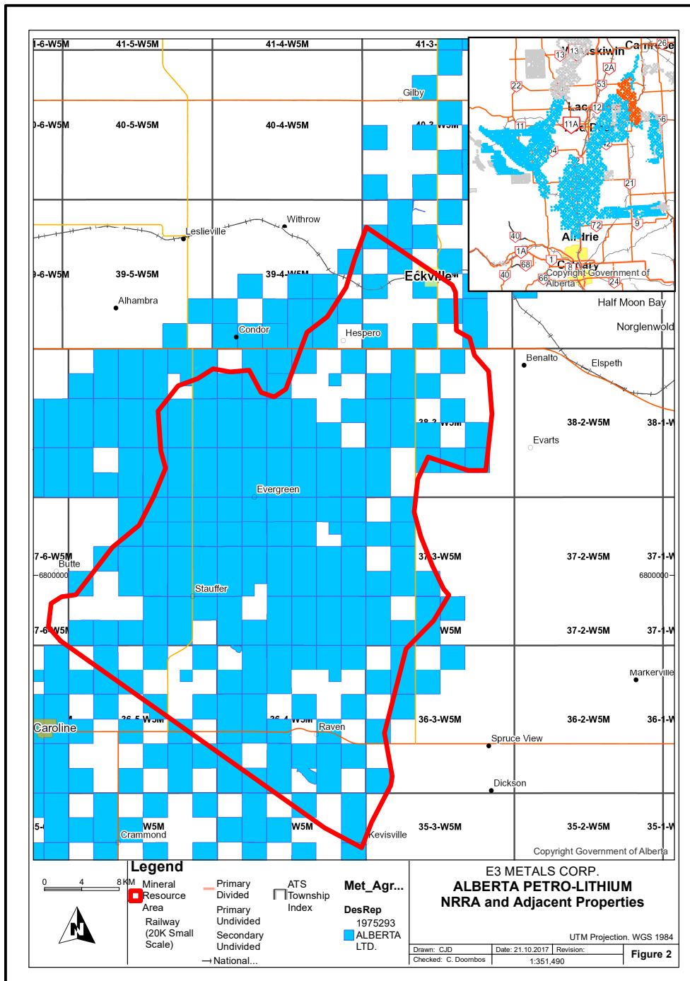
Figure 28. Area map showing the location of E3 Permits and surrounding permits. Permits in blue are held by 1975293 AB Ltd. a wholly owned subsidiary of E3 Metals. White squares interspersed among the blue permits indicate Freehold (individual or corporation) interest.
