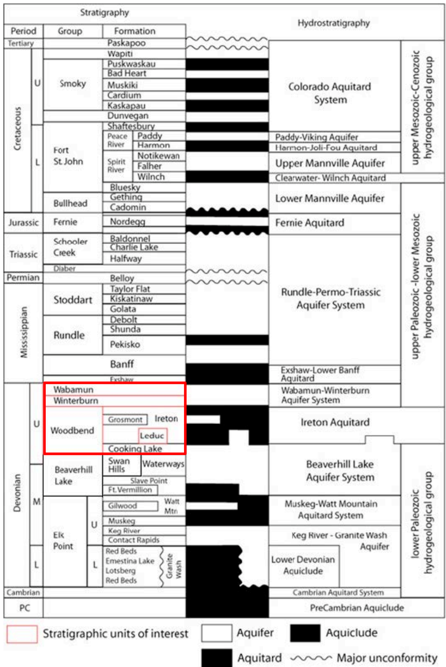
Figure 7: Regional stratigraphy/hydrostratigraphy of Alberta (adapted from Hitchon et al., 1990). The stratigraphic units of interest are denoted in red.
