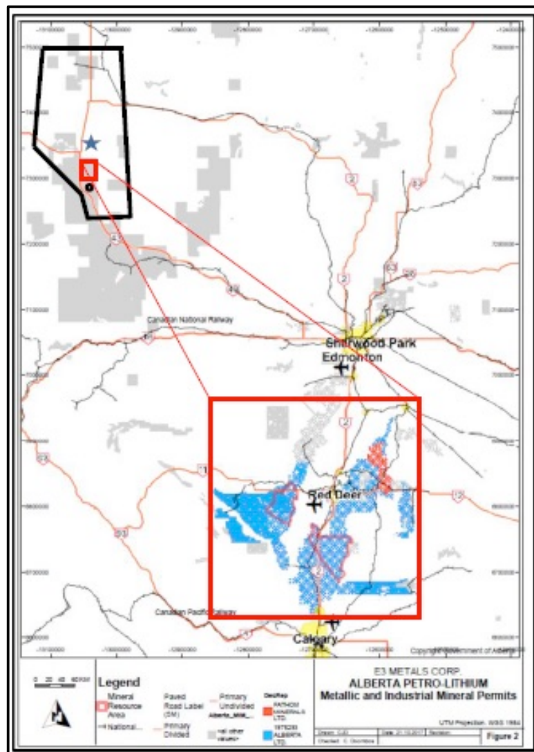
Figure 1. Location of Alberta Petro-Lithium Project in south-central Alberta (E3 Metals, 2017)
