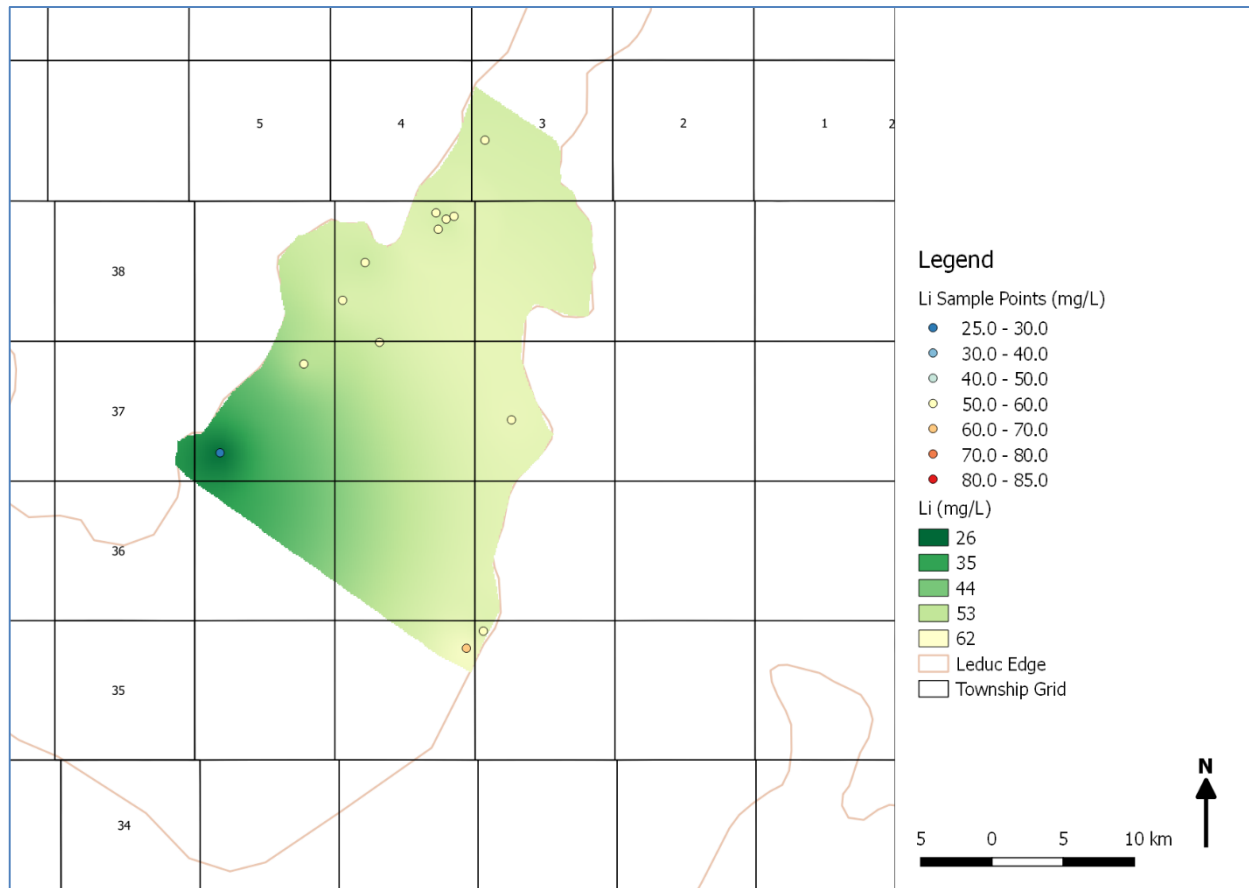
Figure 27. Kriged lithium concentrations in the NRRR. The color ramp scale was chosen in order to see trends across the resource area. Interpolated lithium in the NRRR range from 26.7 mg/L to 61.3 mg/L.
