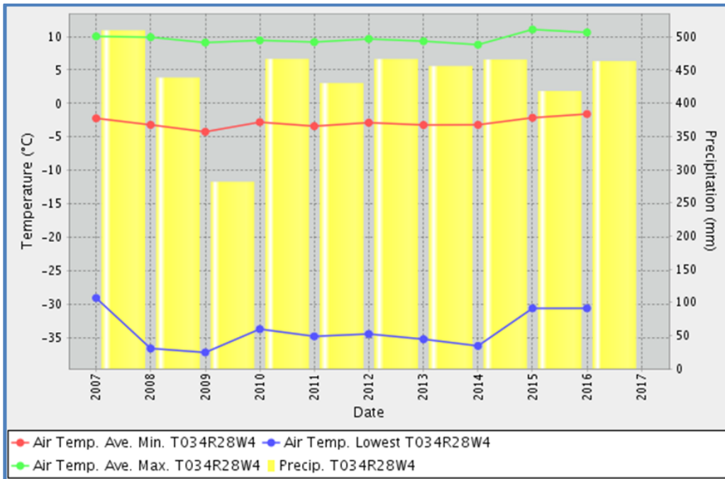
Figure 6. 10-year temperature and precipitation ranges for T34N R28W, the center of the Rocky claims (ACIS, 2017).
